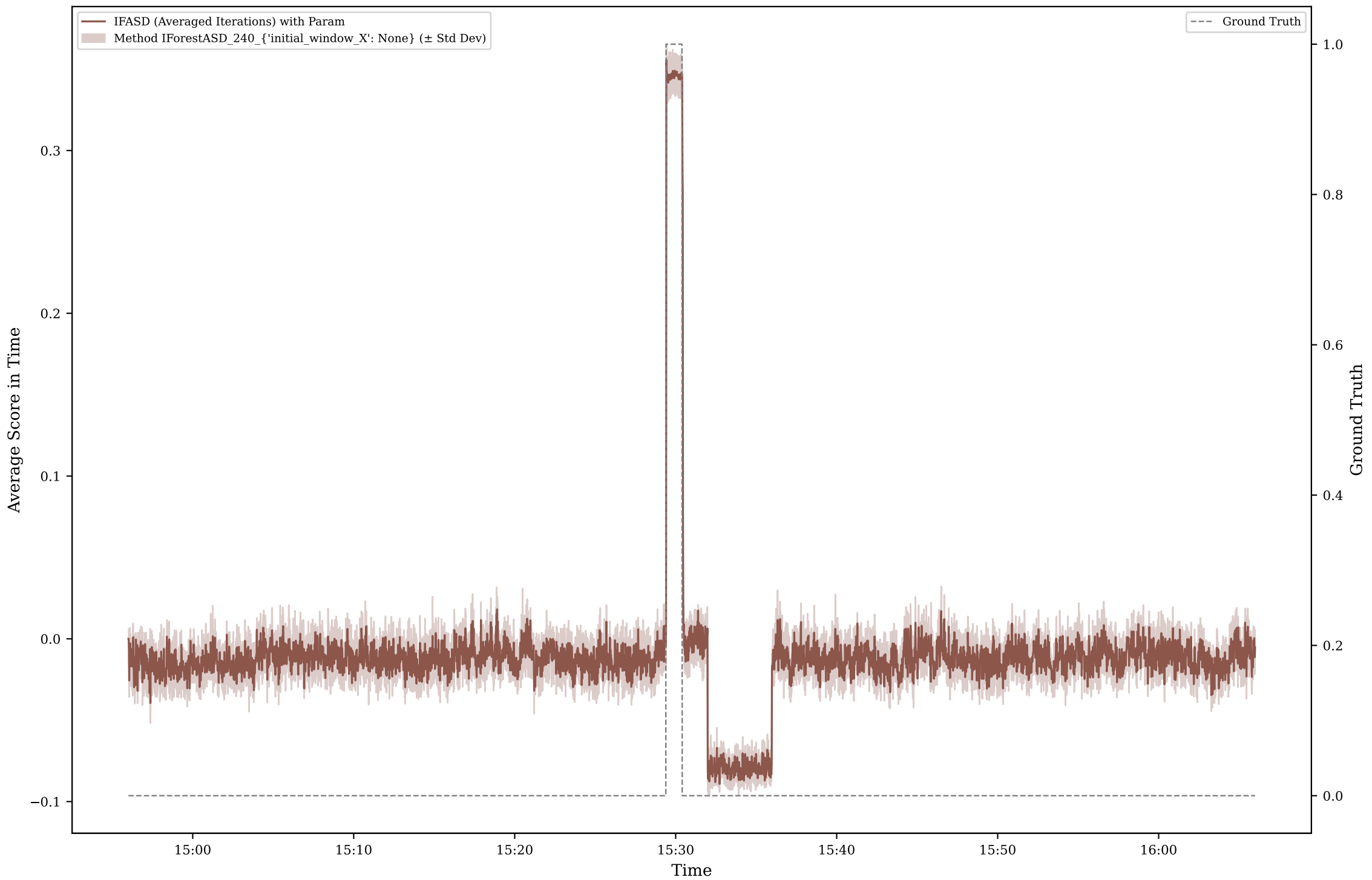
Method IFASD Score for Scenario A1
